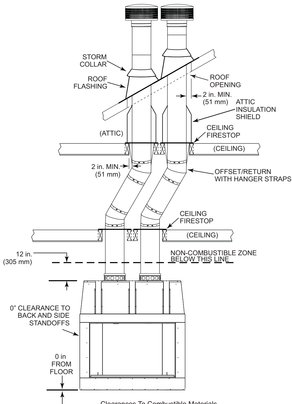
Clearances To Combustible Materials Figure 5
