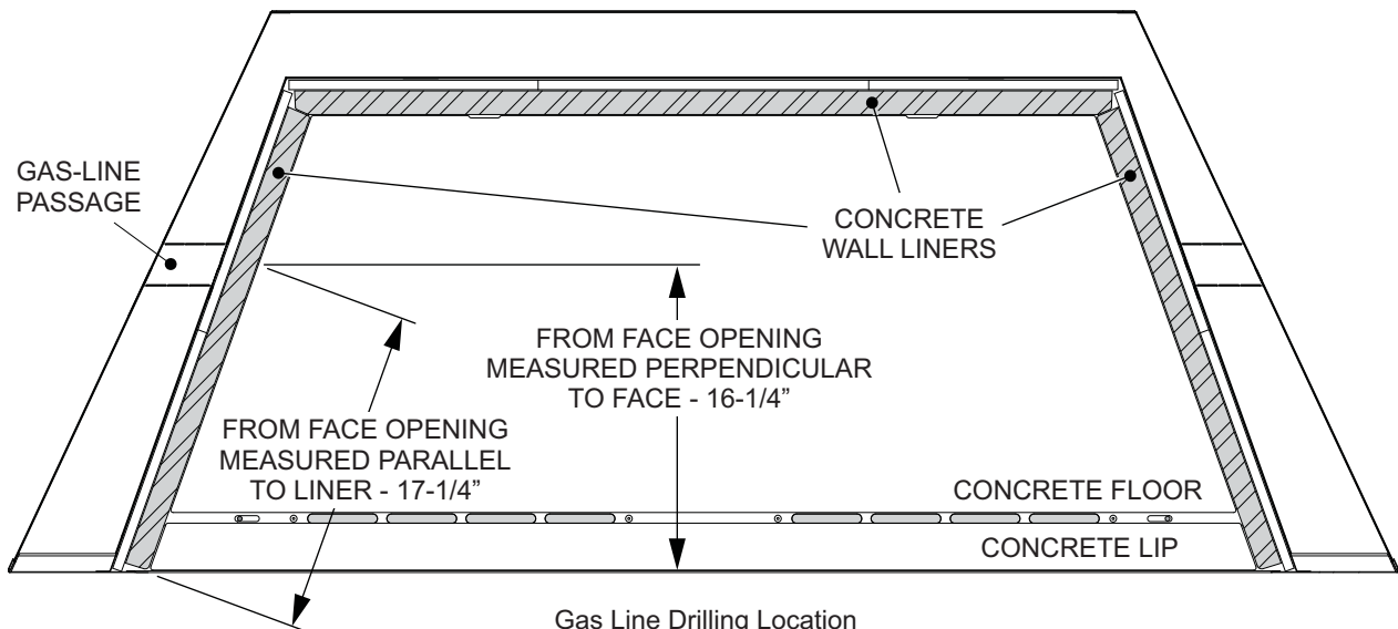
Gas Line Drilling Location Figure 54
