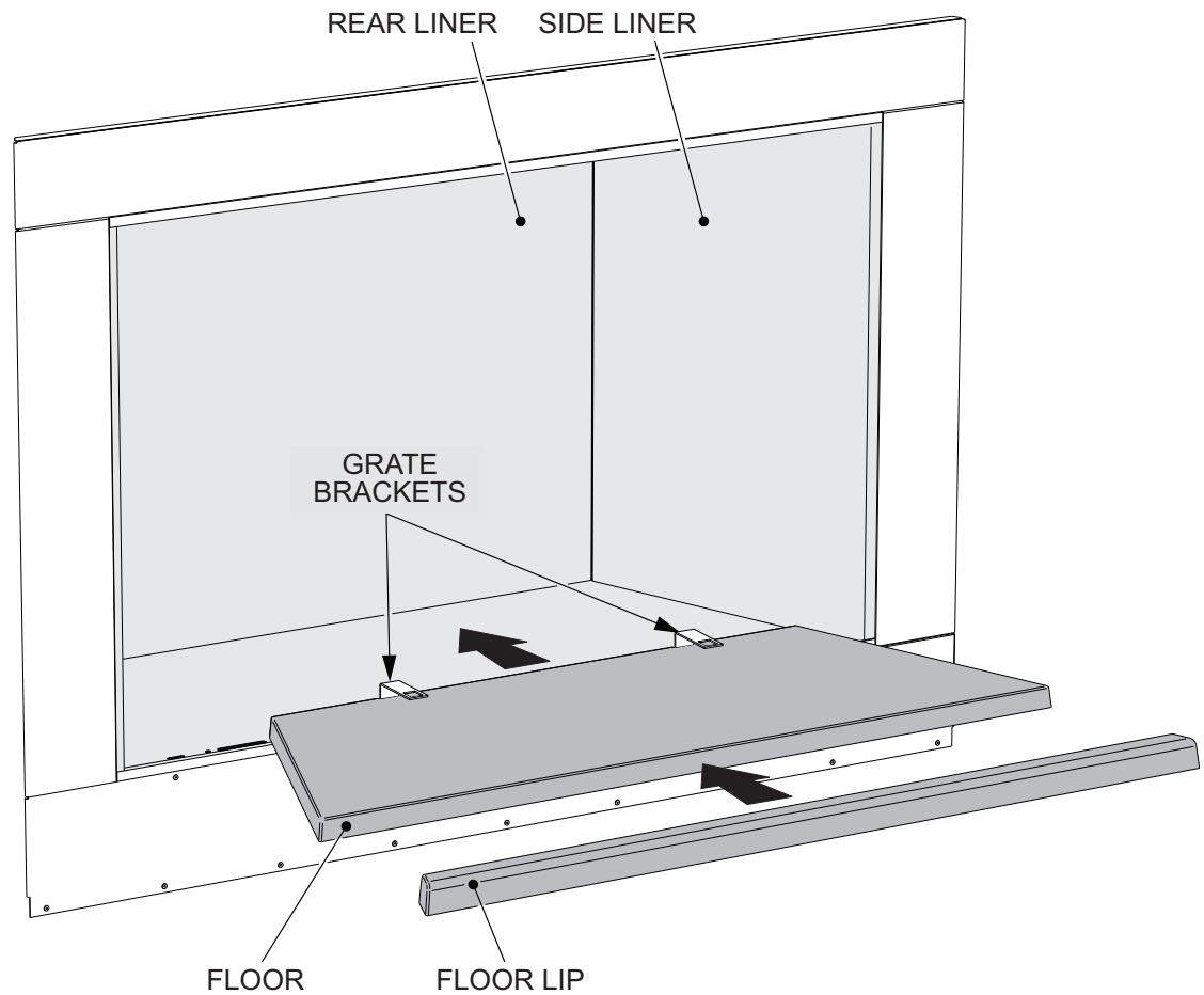
Install Floor and Lip Figure 51
