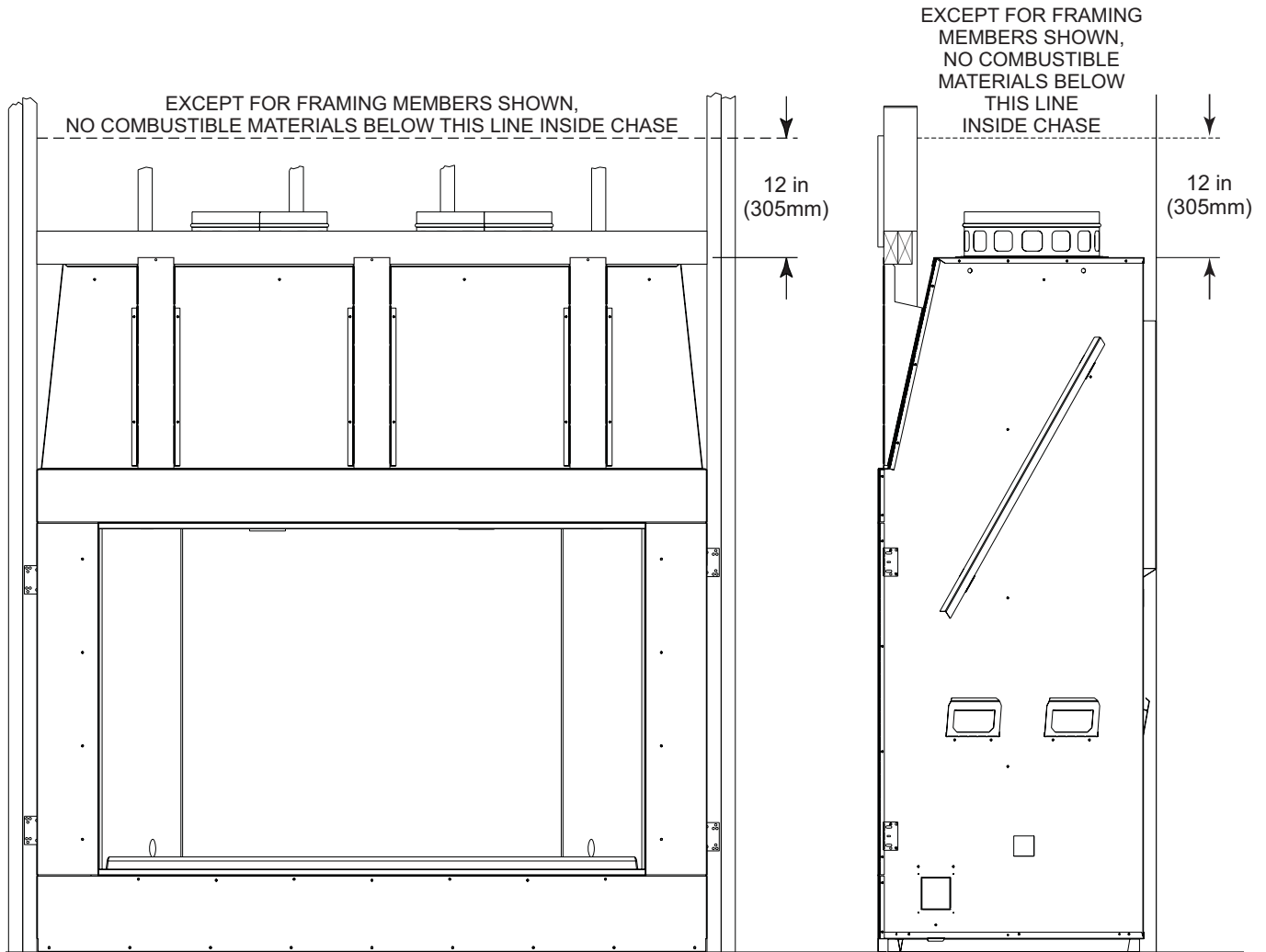
Clearances To Combustible Materials Figure 6
