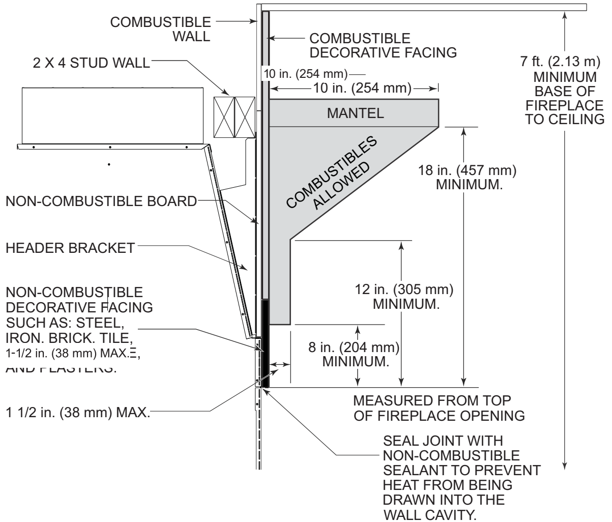
Mantel Specifications Figure 45
