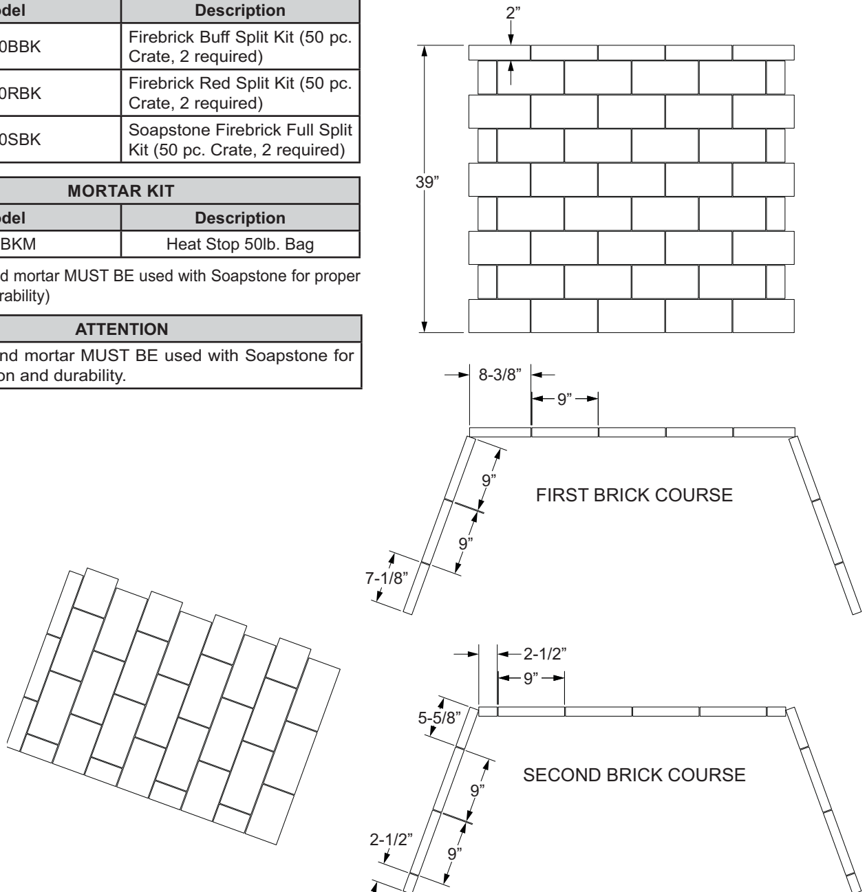
Brick Layout Diagram Figure 50
