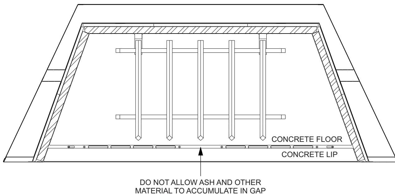
Gap Behind Lip Figure 57
