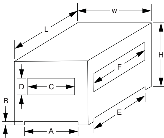
House Shroud Dimensions Figure 32
