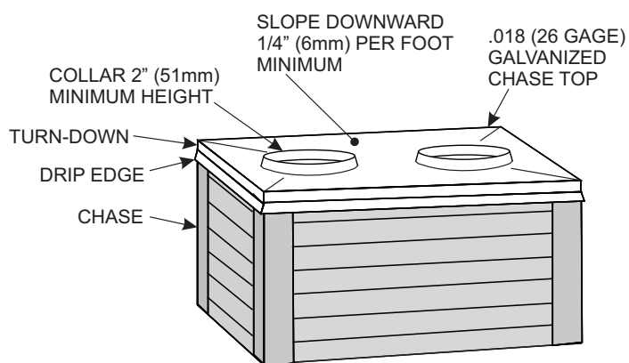
Chase Top Construction Figure 27
