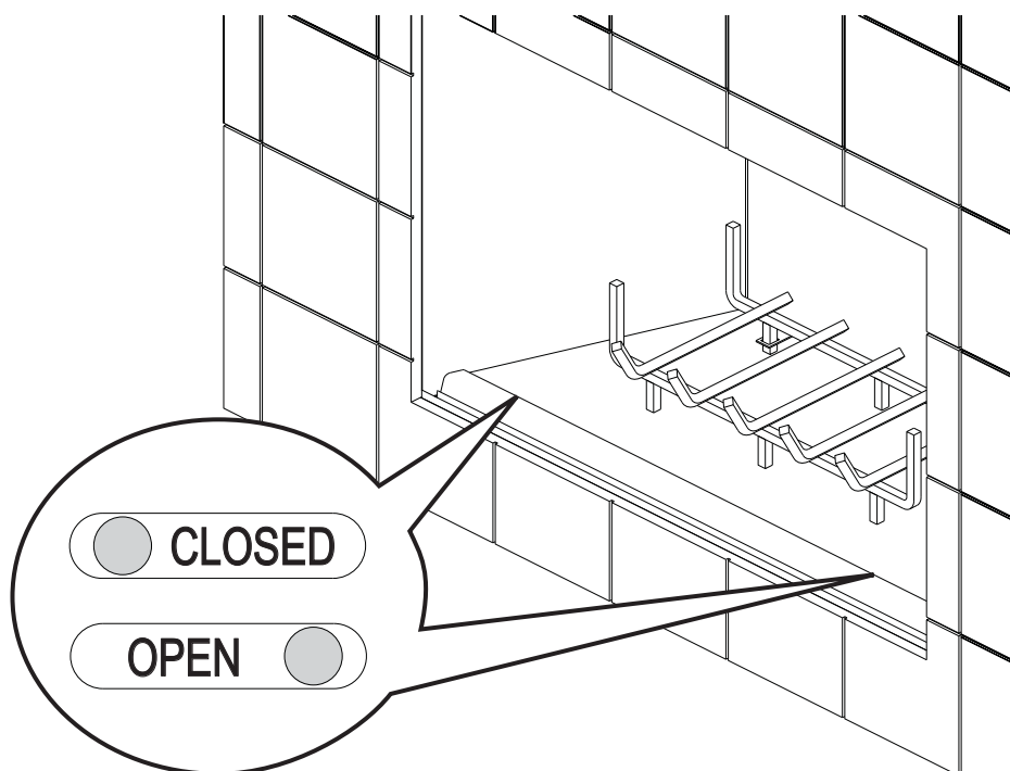
Outside Air Kit Figure 57
