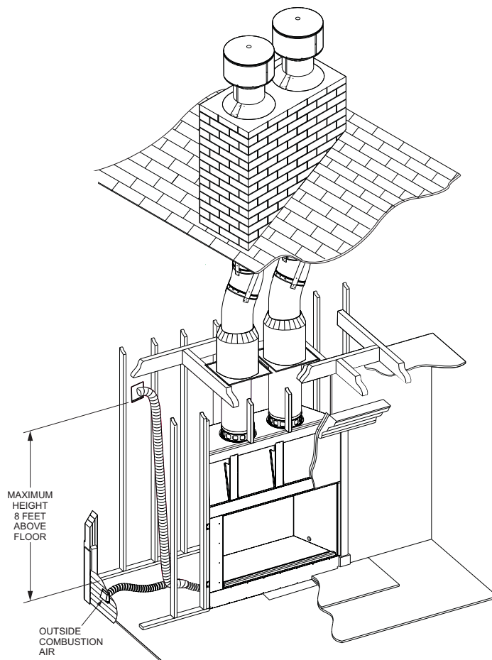
Outside Air Hood Locations - Figure 13
