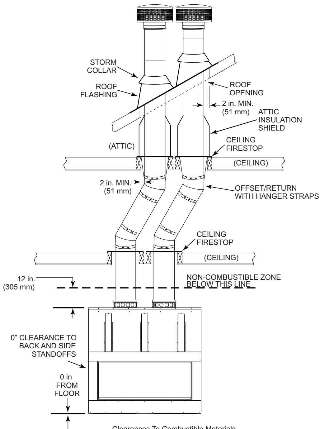
Clearances To Combustible Materials Figure 5
