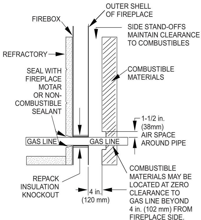
Gas Line Installation Figure 52
