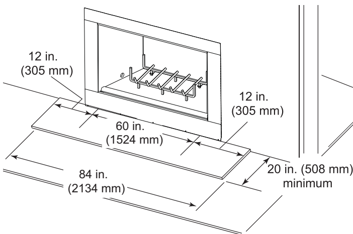
Hearth Extension Dimensions Figure 36
