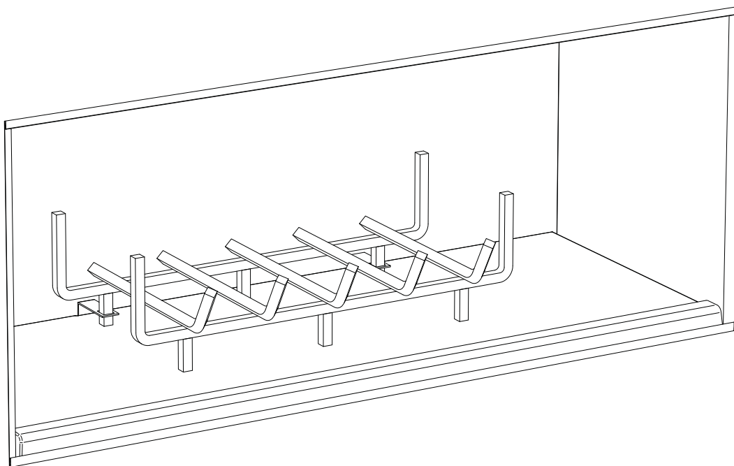
Install Grate Figure 54
