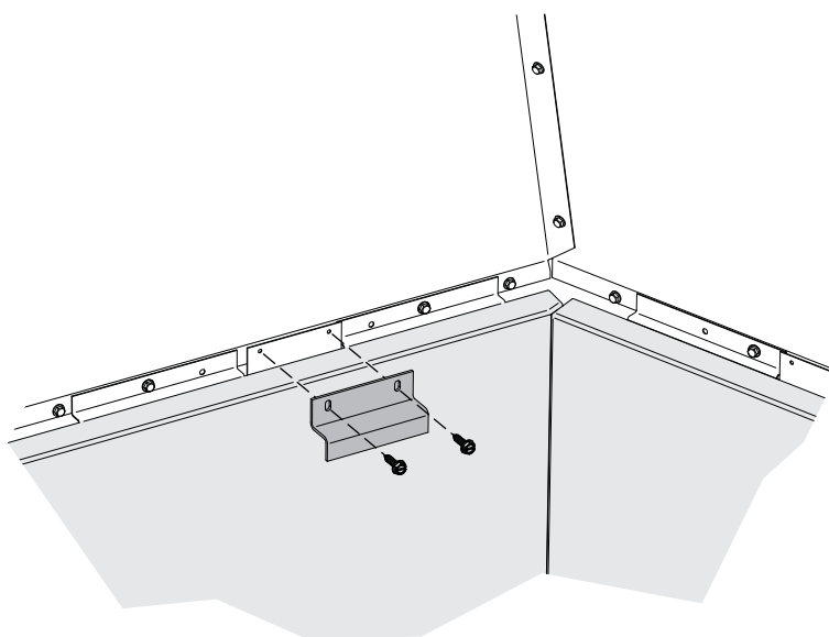
Install Liner Bracket Figure 48
