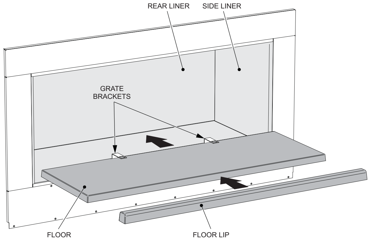
Install Floor and Lip Figure 51
