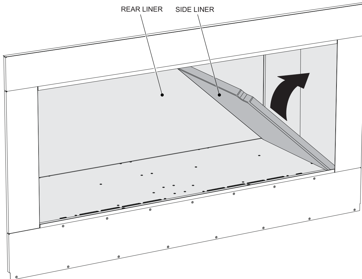
Install Side Liner Figure 49
