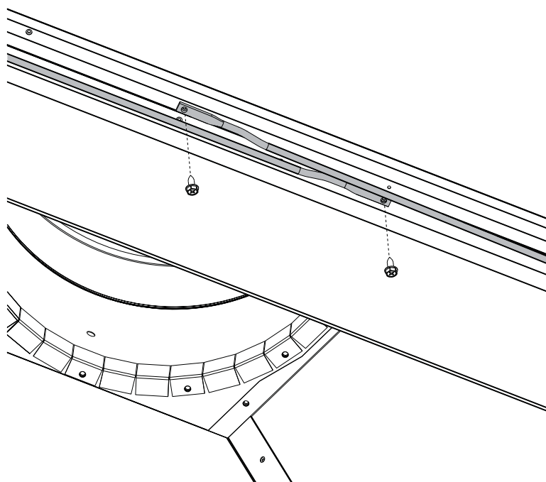
Install Screen Rods Figure 55
