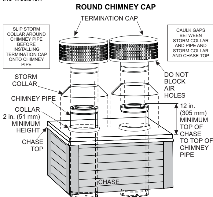
Installing a WB12VRCC Round Termination Cap Figure 28
