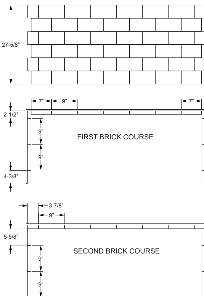
Brick Layout Diagram Figure 50
