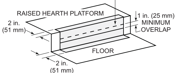
Protect The Front Of A Raised Platform Figure 11
