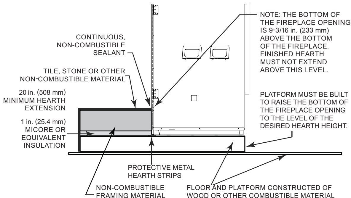
Raised Hearth Extension and Fireplace Framing Materials Figure 42
