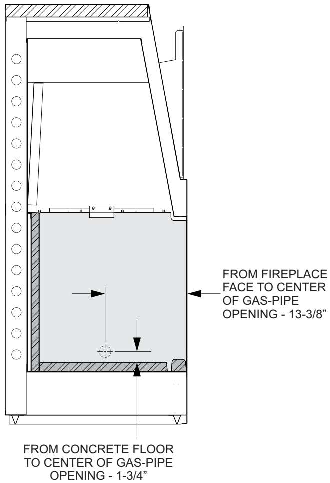
Gas Line Location Figure 53
