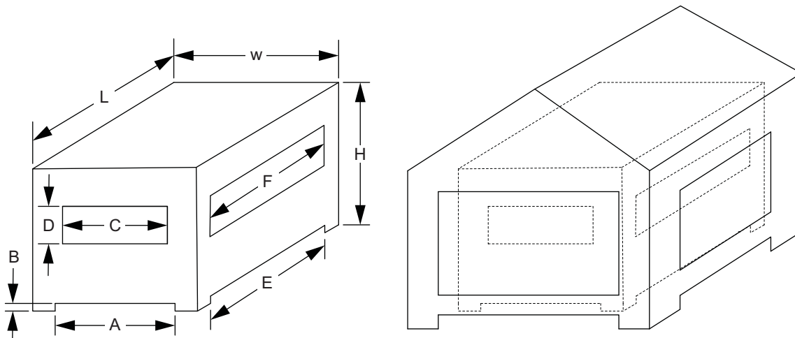
House Shroud Dimensions Figure 32
