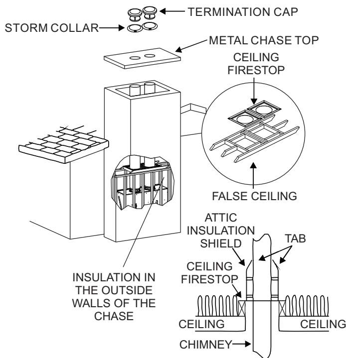
Chase Assembly - Figure 7
