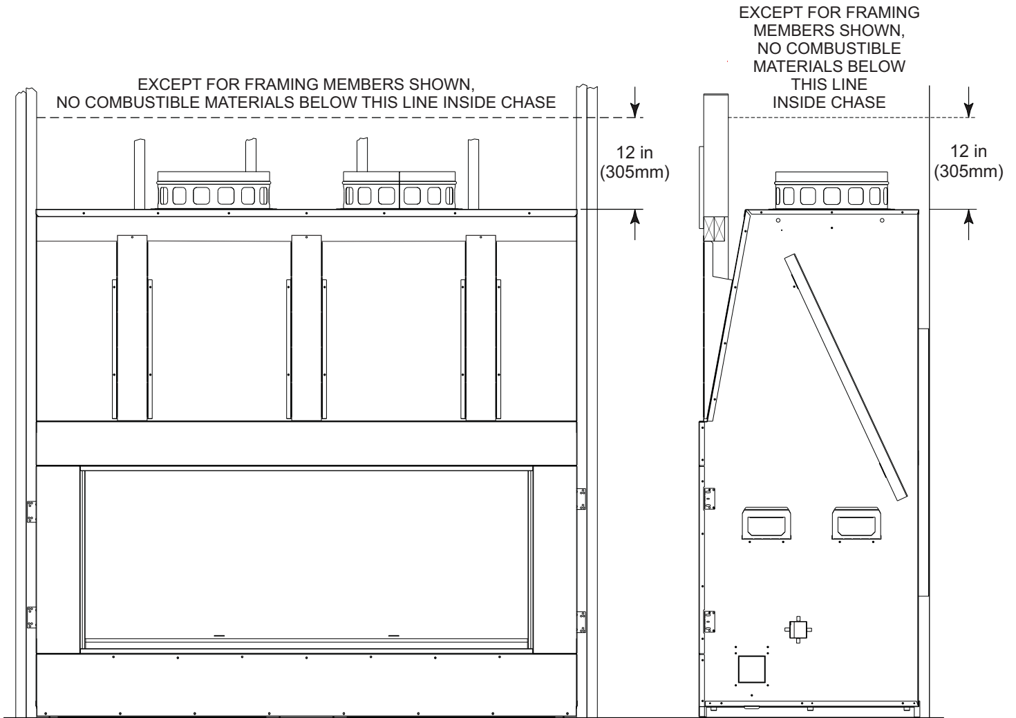
Clearances To Combustible Materials Figure 6
