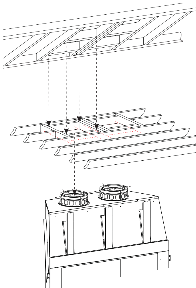
Ceiling/Attic Construction Figure 26
