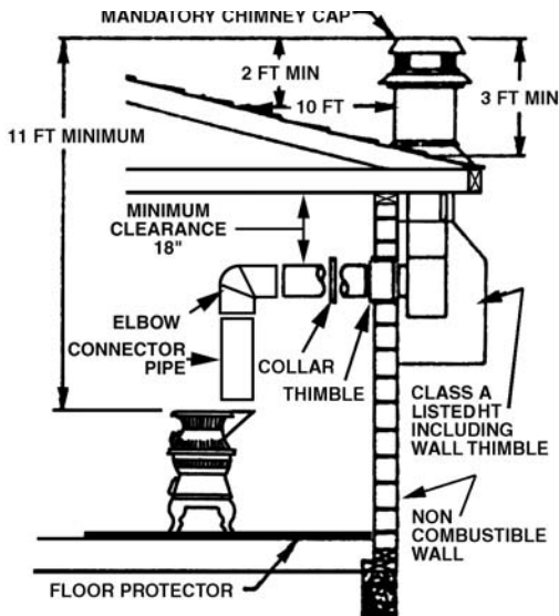
Fig. 12 - Chimney Connection to Fireplace Through Masonry Wall
