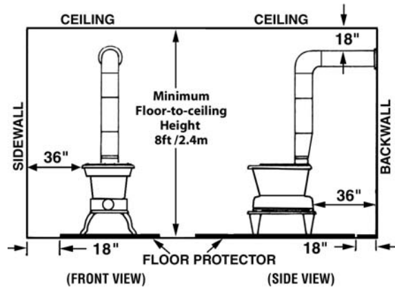
Fig. 2 Minimum Clearance Dimensions from Combustible Surfaces Fig. 3
