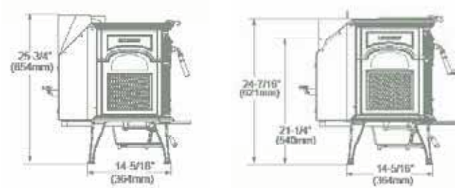
Side - Top Vent
