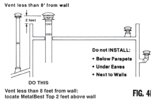
FIG. 4 - RAIN CAP LOCATION RULES
