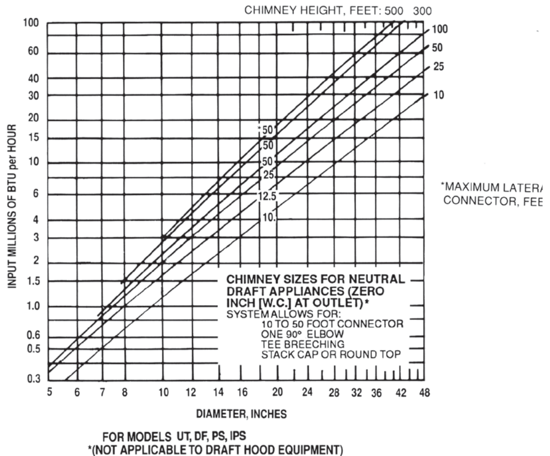
FIG. 32 - CHIMNEY SIZES FOR NEUTRAL DRAFT EQUIPMENT
