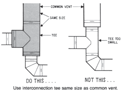
FIG. 16 - PROPER TEE SIZE FOR INTERCONNECTION
