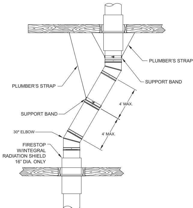
FIG. 12C (16" Diameter)
