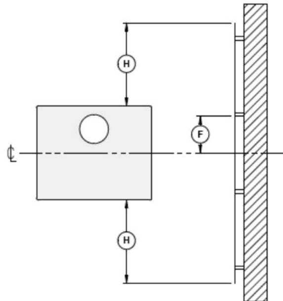
Figure 23: Heat shield clearances
