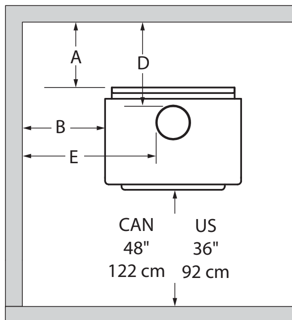
Clearances - Top
