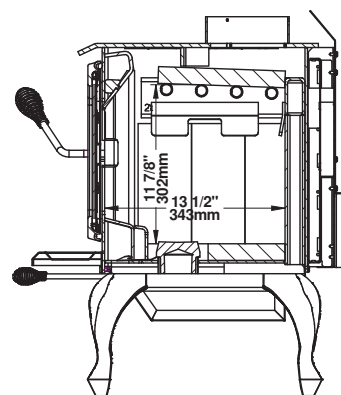
Combustion chamber - side view
