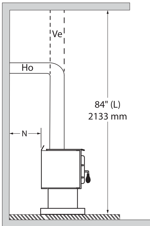
Clearances - Ceiling
