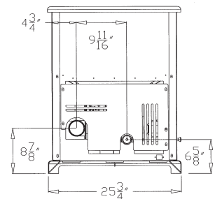
Home Heater with optional 17.5" hopper extension
