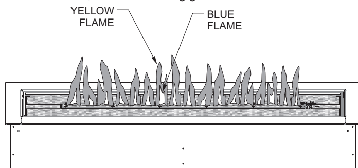
Figure 33 - Correct Flame Propane
