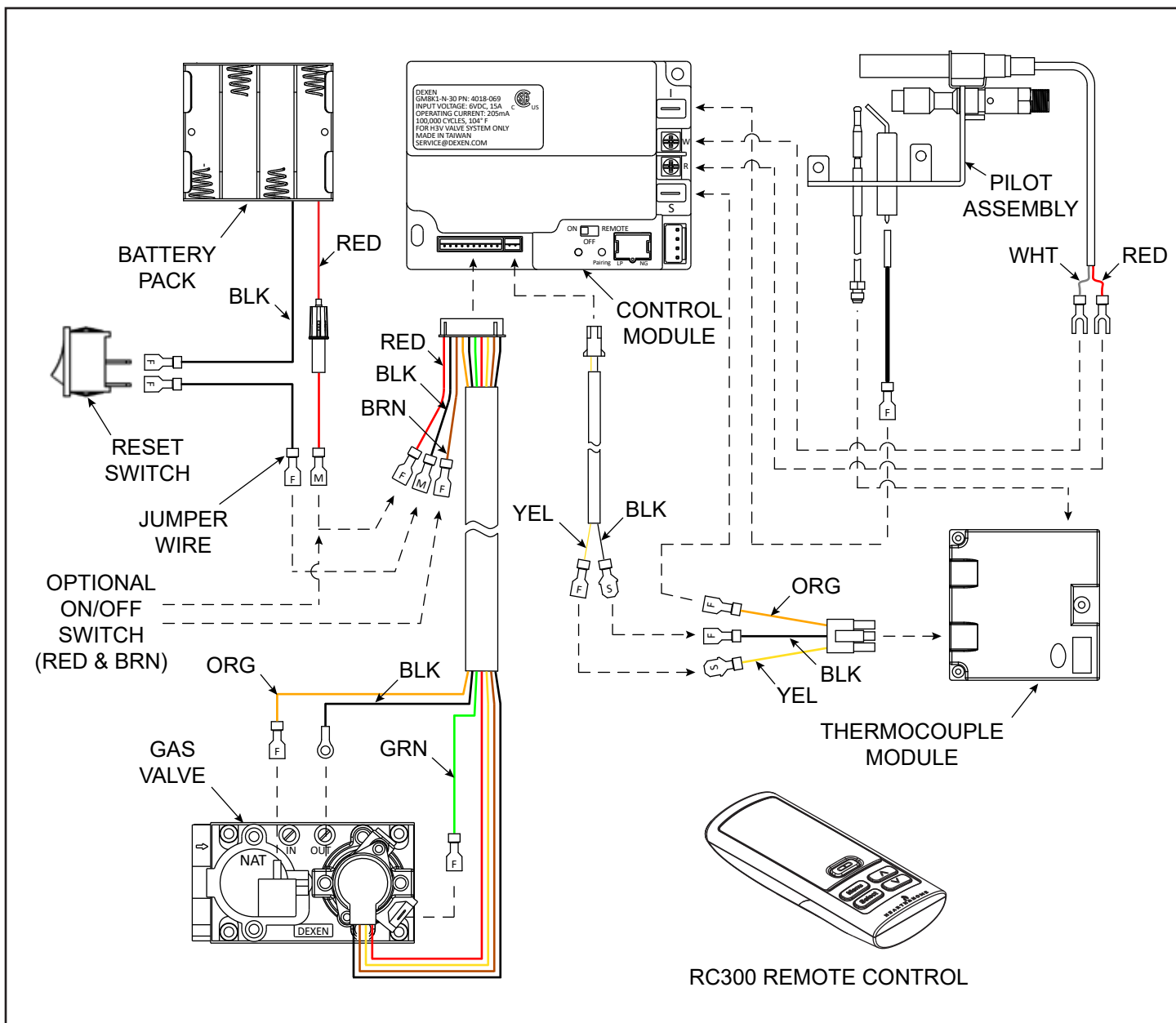
Figure 8.4 Intellifire™ Plus (IPI) Wiring
