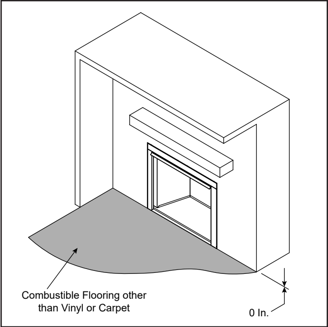
Figure 5.4 Combustible Flooring
