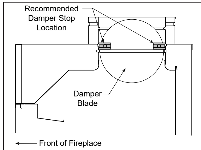
Figure 6.1 Factory-Built Fireplace
