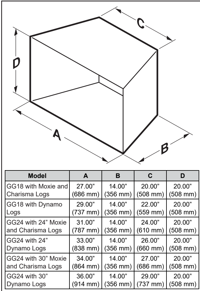
Figure 3.1 Minimum Hearth Dimensions
