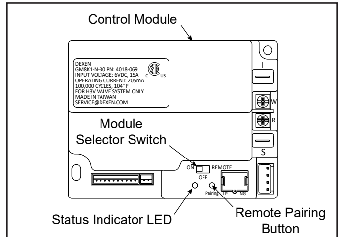
Figure 8.2 Control Module
