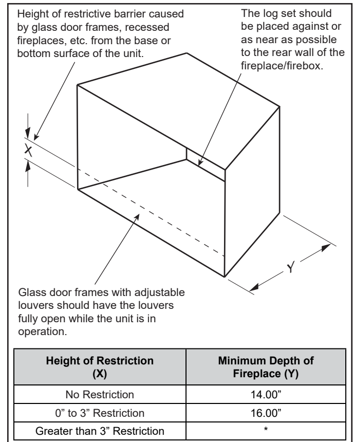
Figure 3.2 Restrictive Barriers
