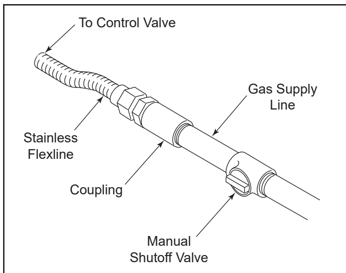
Figure 7.1 Gas Connection
