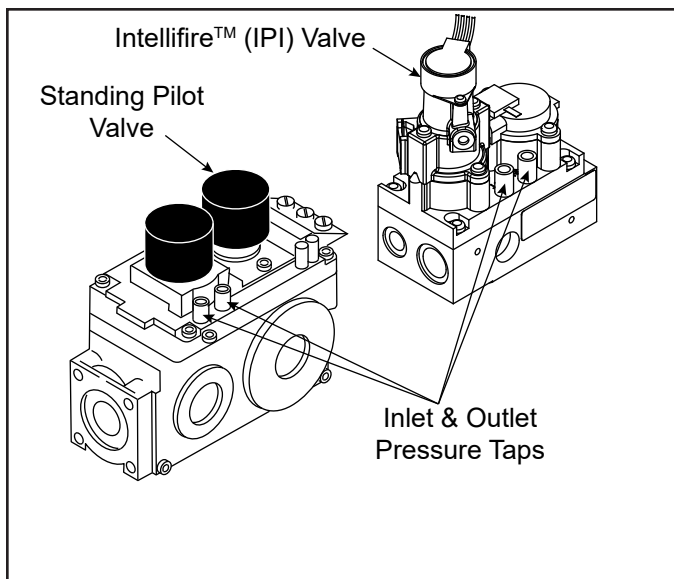
Figure 7.2 Pressure Taps
