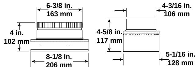
DVP-2SL Adapter
